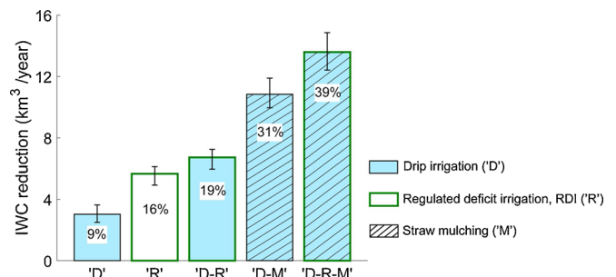
Fig. 1. Annual average reduction of irrigation water consumption (IWC) in maize cultivation in China under five scenarios of improved on-farm water management. Bars refer to the absolute annual average IWC reduction (km 3 /year) for maize, with the relative change (%) compared with BAU, indicated by the number inside each bar. Whiskers indicate the extent of inter-annual variations of simulated IWC reduction during 1995–2014.
